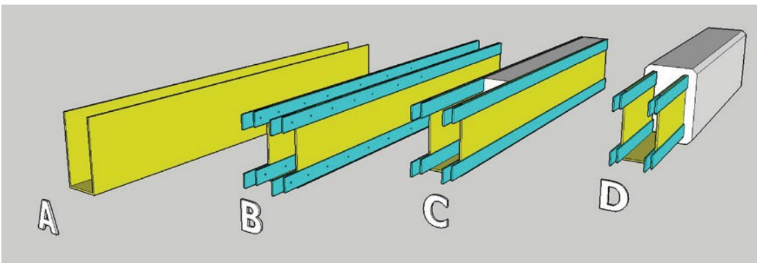
Construction of the arch ribs. (A) Sheet piling bent to a trough shape on land. (B) Steel plates bolted to sheet piling trough for strength and then winched across the gorge in 4 sections. The 4 sections then bolted together to form a continuous arch. (C) Concrete infill placed inside the trough. (D) Render applied to external surfaces to complete the arch ribs.
